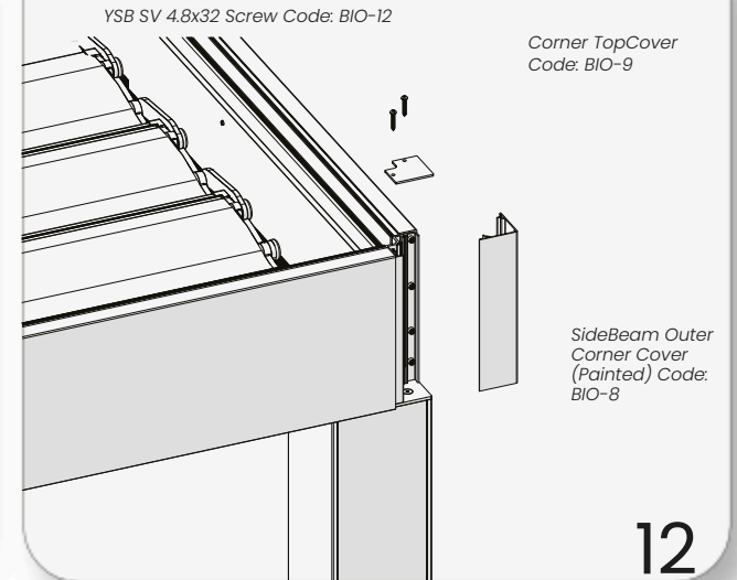
YSB SV 4.8x32 Screw Code: BIO-12
